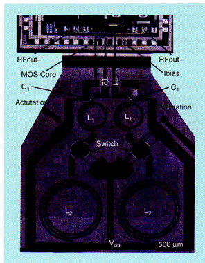
Figure 11. MEMS enabled RF signal source (MEMS-CMOS oscillator) [18].
