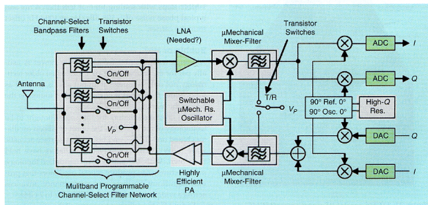
Figure 9. Typical RF MEMS replacing devices (Shaded) in TxRx section of handsets [6].
