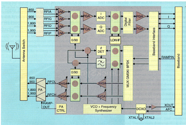
Figure 2. GSM transceiver chipset with on-chip DCXO [2].
