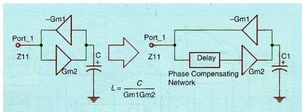
Figure 12. A typical representation of gyrator-based active.
