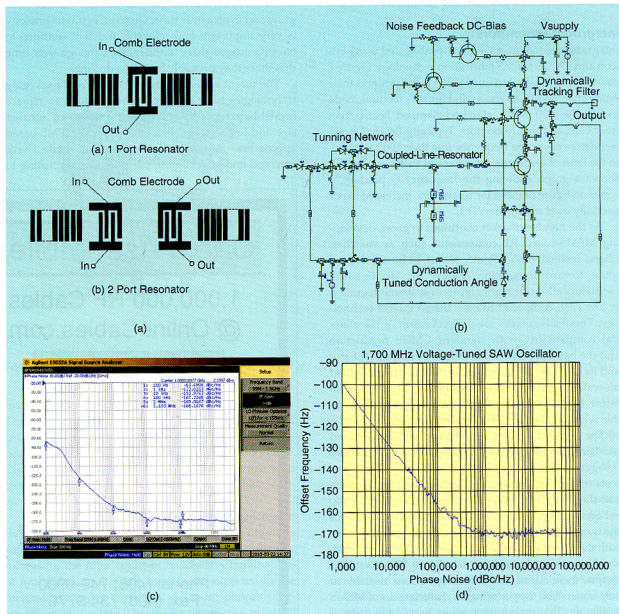
Figure 6. (a) SAW resonator, (b) typical schematic 1 GHz VCSO (patented), (c) measured phase noise plot of 1 GHz VCSO, and (d) measured phase noise plot of 1.7 GHz VCSO with latest technological advancements in tiny size (0.4 × 0.4 inches).
