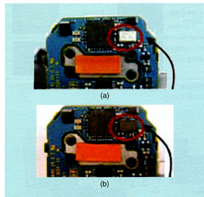
Figure 10. Typical quartz and MEMS oscillator. (a) 67.5 MHz quartz oscillator, and (b) 67.5 MHz MEMS oscillator.
