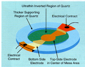
Figure 3. A typical inverted high-frequency Mesa quartz resonator [3].
