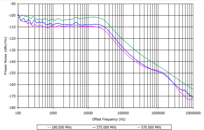
Phase Noise
