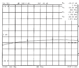
KEK-706H (COUPLING)
