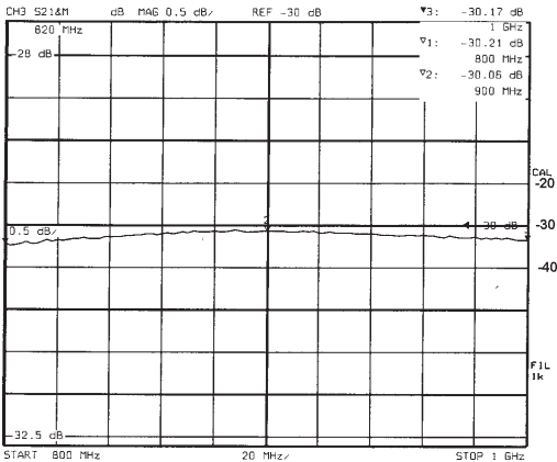
KEK-704DH (COUPLING)
