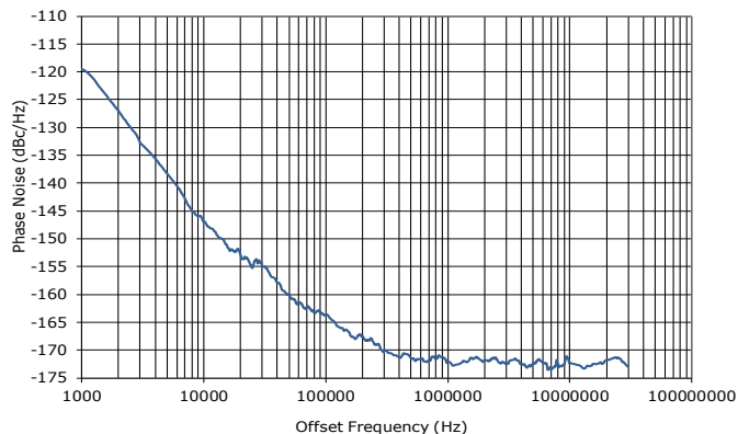
Phase Noise
